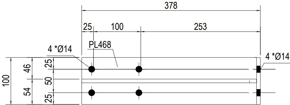
FRONT VIEW
